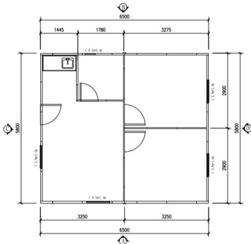
Layout plan
